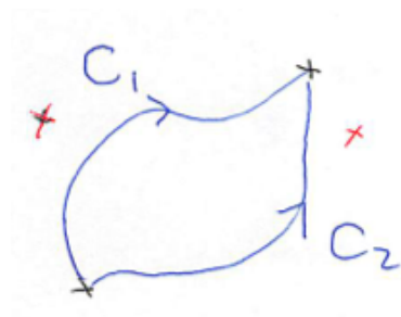
図 35: \int_{C_1} f(z) dz = \int_{C_2} f(z) dz
