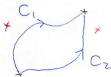
図 21: \int_{C_1} f(z) dz = \int_{C_2} f(z) dz
